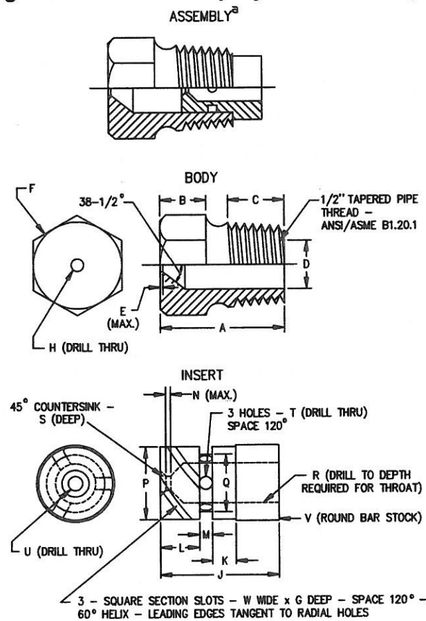
Figure 1 – Rain-Test Spray Head Drawing
